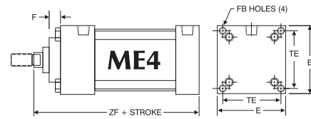
'MF1', 'MF2' Flange & 'ME3', 'ME4' Cap Mount Dimensions
