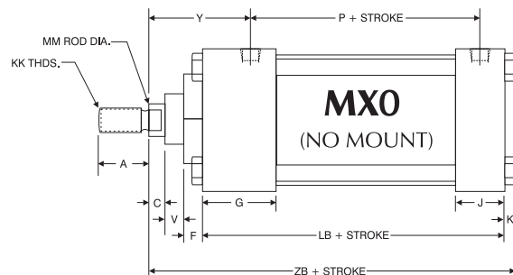
Basic Dimensions 'MX0' Standard & Oversize Rods
