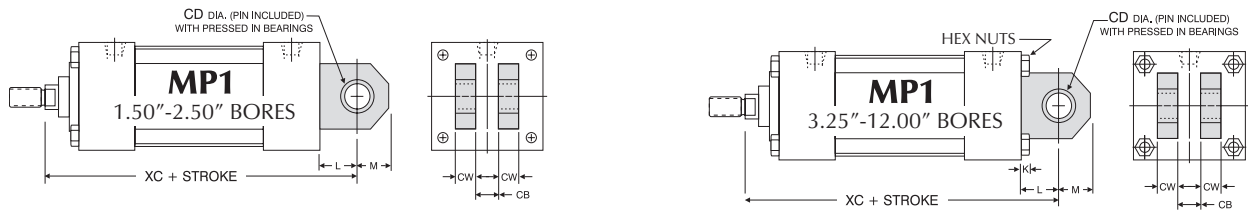
Extruded MP1 Mount (Extruded: 1.50" - 8.00" Bores, Weldment: 10.00" & 12.00" Bores)
