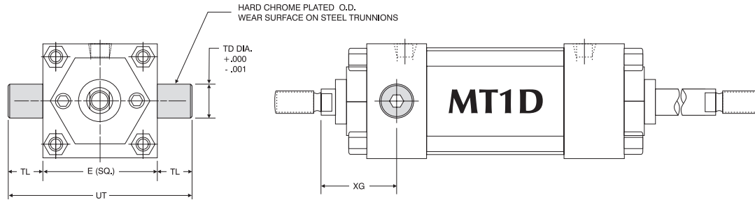
Double Rod End 'MT1D' Head Trunnion Mount Dimensions
