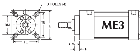
'MF1', 'MF2' Flange & 'ME3', 'ME4' Cap Mount Dimensions
