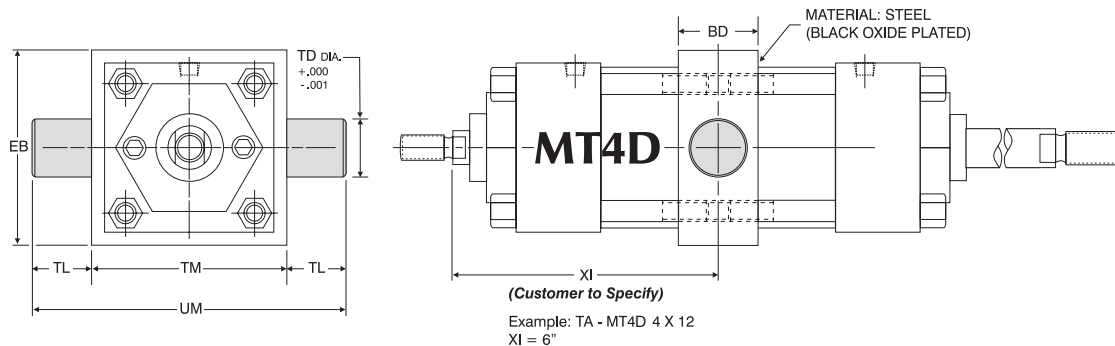
Double Rod End 'MT4D' Intermediate Trunnion Mount Dimensions
